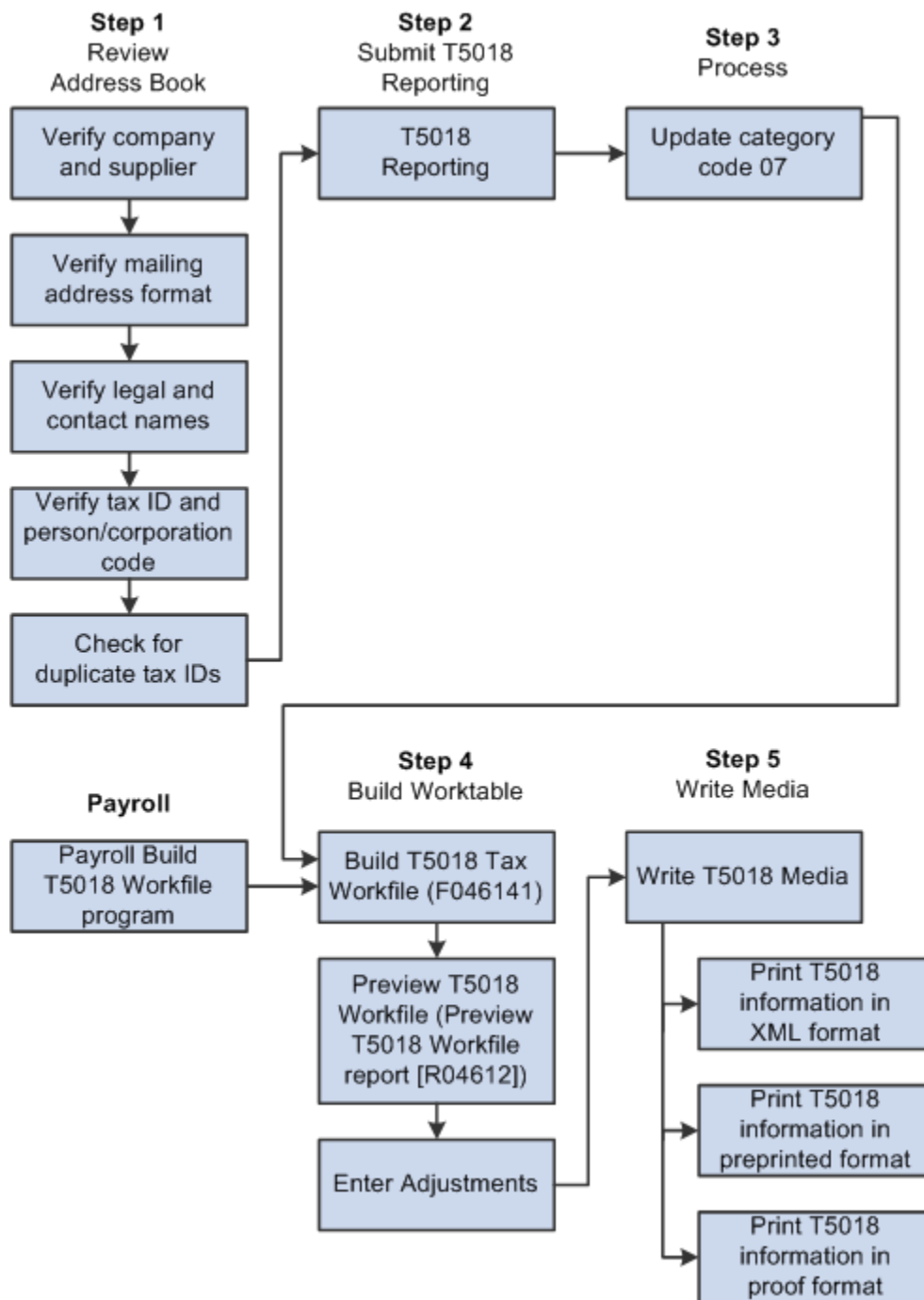
Figure 18–1 Process Flow for T5018 Processing
