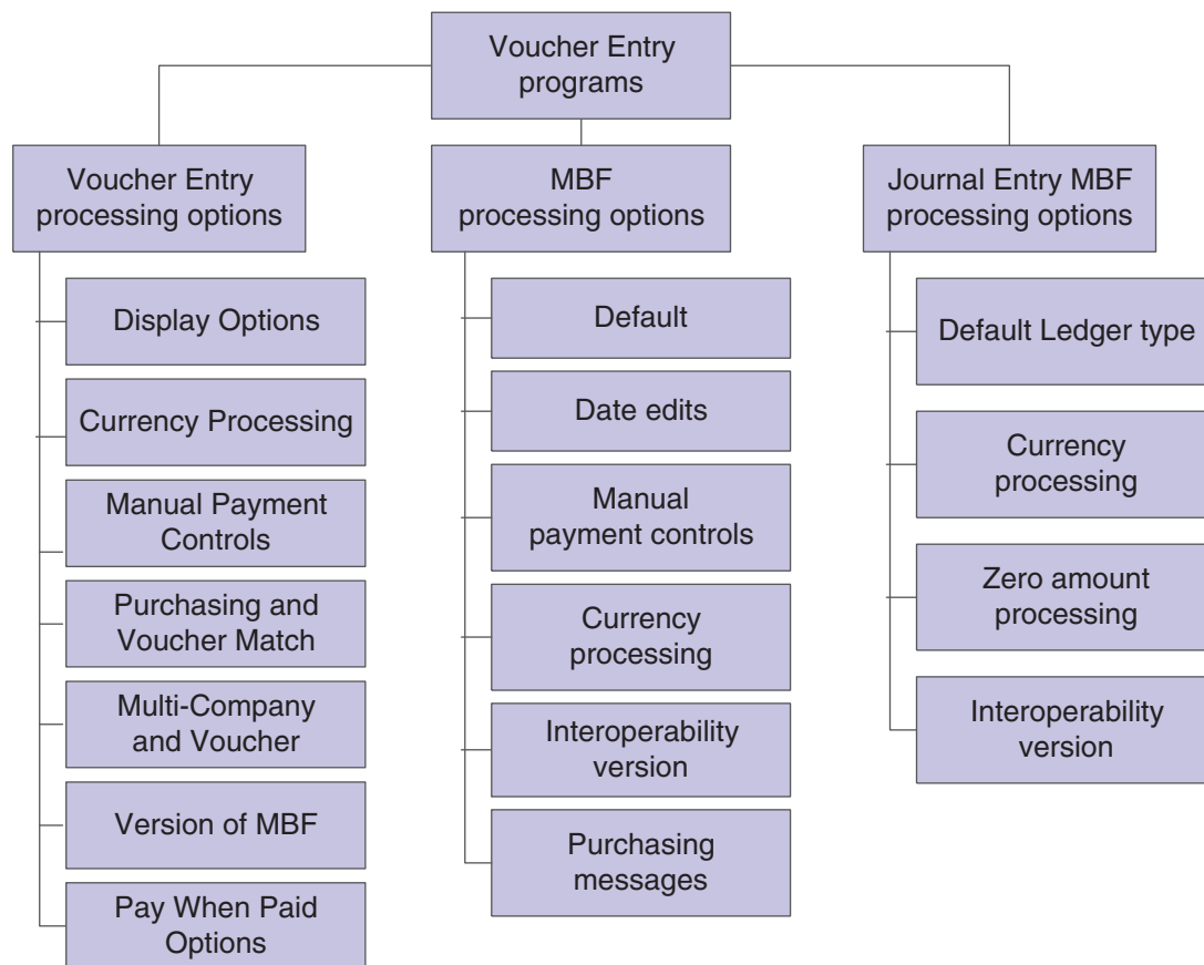
Figure 6–2 Processing options for voucher entry
