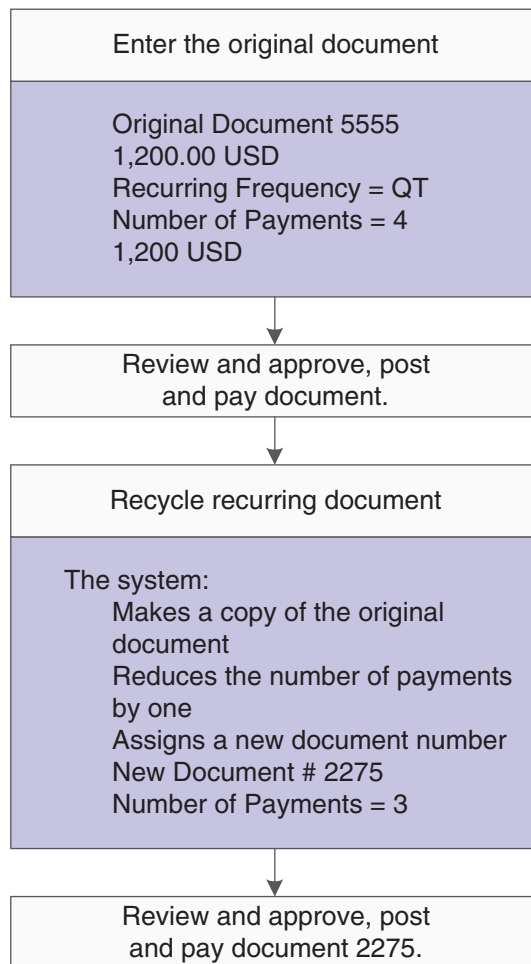
Figure 6–7 Processing recurring invoices and vouchers
